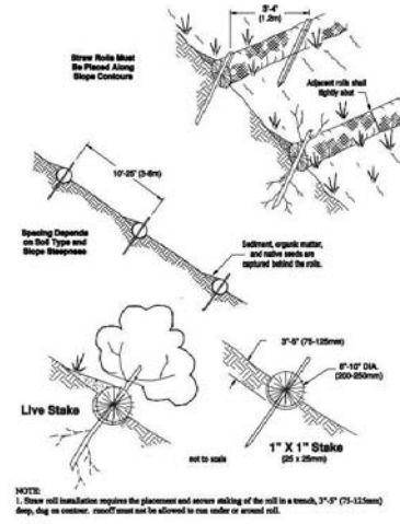
STRAW WATTLE INSTALLATION NTS
